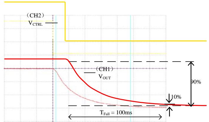
V_CTRL: 0.25V ~ 5V V_OUT: 340V ~ 7000V
