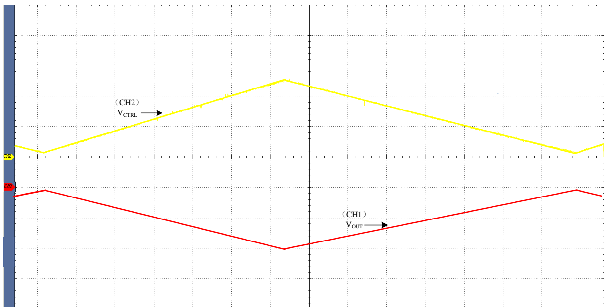
CH1: 2500V/Div CH2: 2V/Div M: 500ms V_CTRL: 0.25V ~ 5V V_OUT: -40V ~ -5000V
